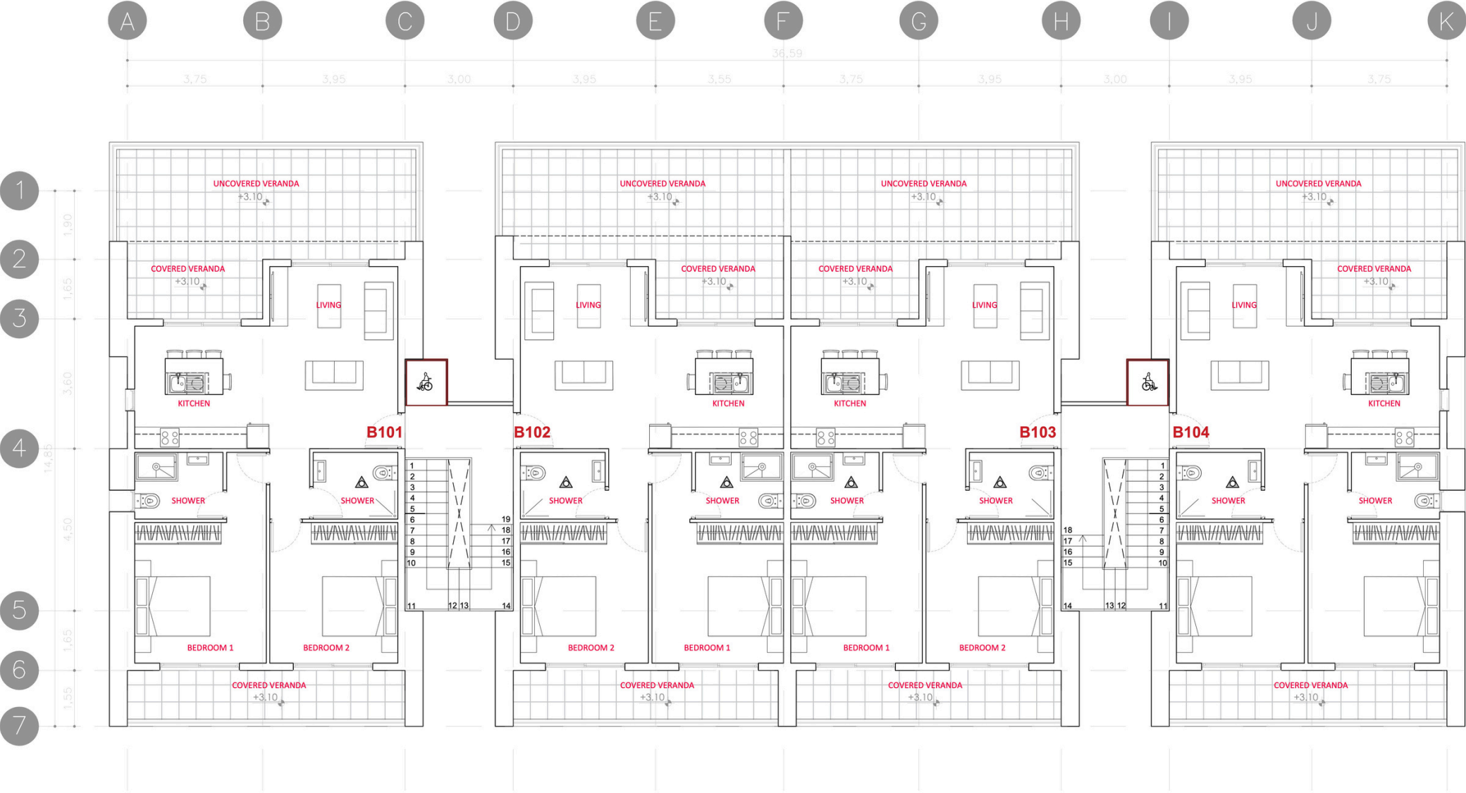
FIRST FLOOR
