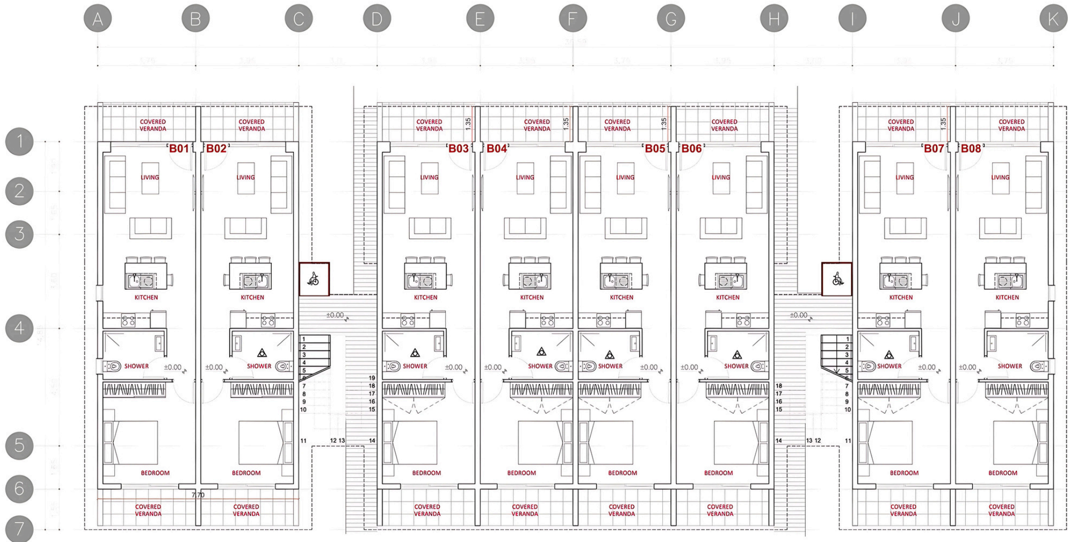
GROUND FLOOR
